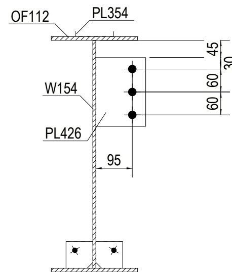
SEC C 1:10
